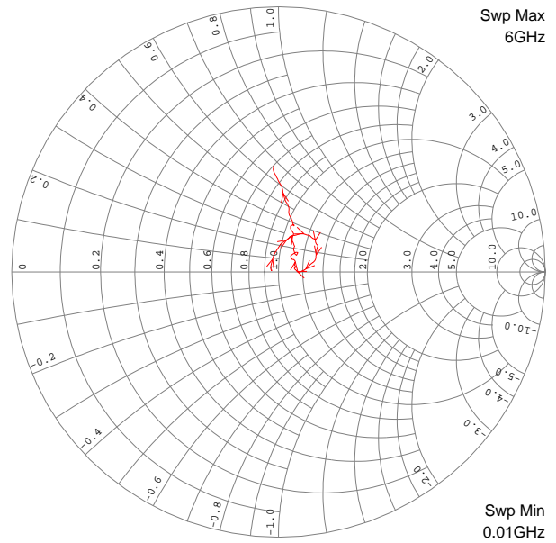
De-Embedded S22, V_{CC} = 4.84\text{V} , I_{CC} = 65\text{mA} , T = 25^\circ\text{C}
