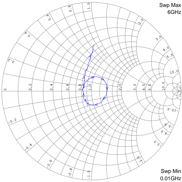
De-Embedded S11, V_{CC} = 4.84\text{V} , I_{CC} = 65\text{mA} , T = 25^\circ\text{C}
